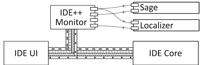
Figure 2: To support developer-aware applications, IDE++ captures and republishes interactions between a developer and an IDE.
